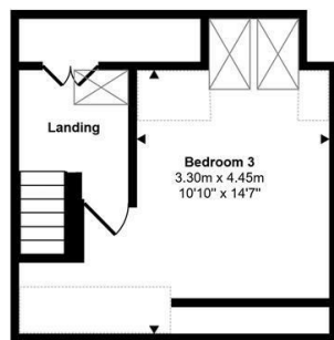
Second Floor Approx 28 sq m / 305 sq ft
